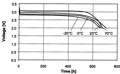
Temperature performance Load 16.2kΩ
