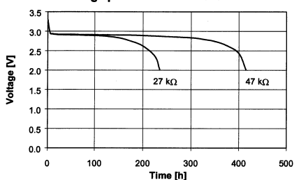
Discharge performance at 23°C
