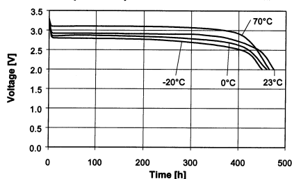
Temperature performance Load 27kΩ
